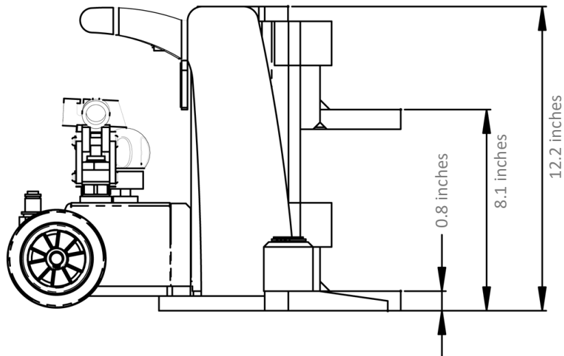
Side Views
