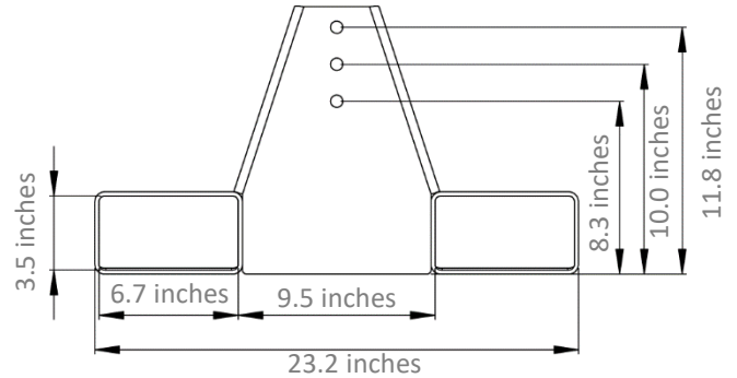
Rear Views
