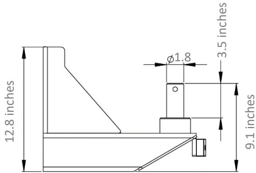
Side Views
