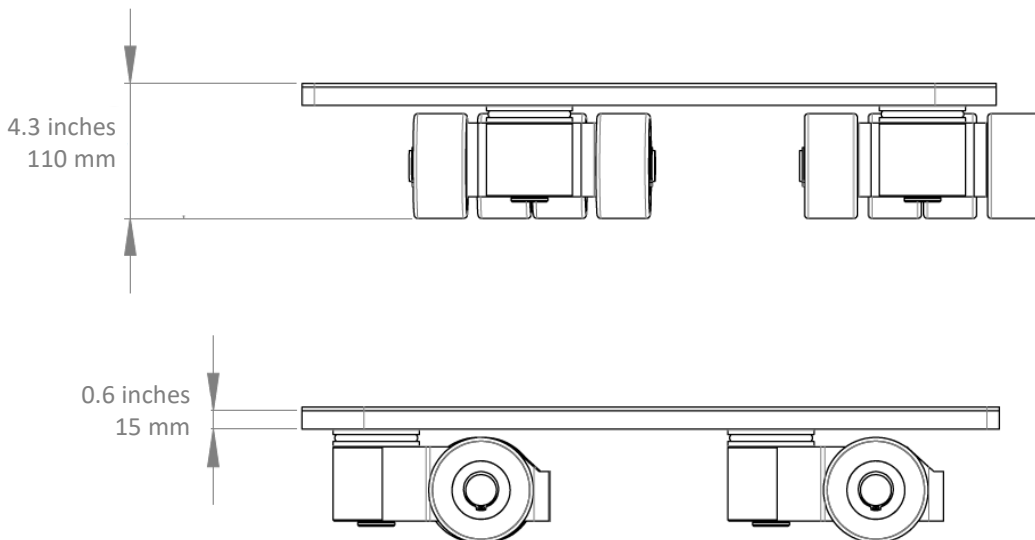
Side Views
